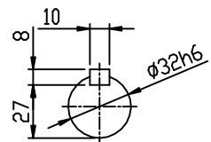
OUTPUT SHAFT
